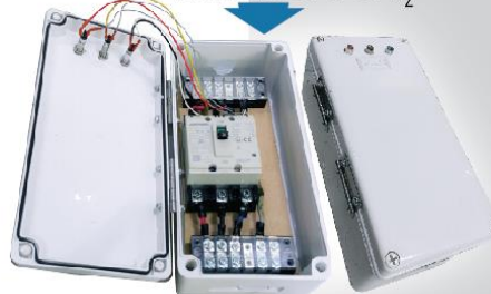
CIRCUIT BREAKER THREE PHASE 380 V. 50 H 2
